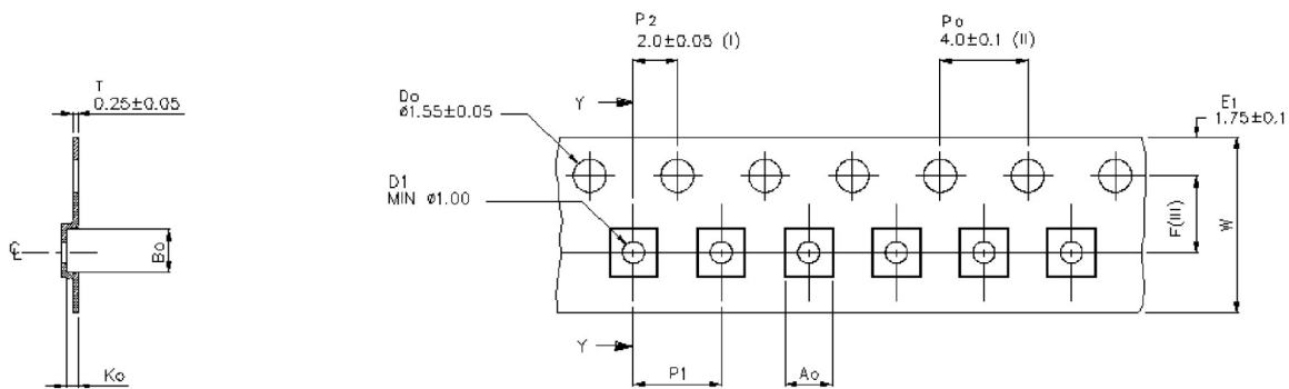
SECTION Y-Y
