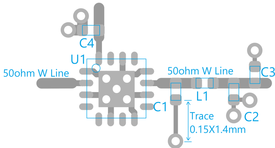
Figure 4: 8TR8211C Reference Design Schematic and PCB Layout
