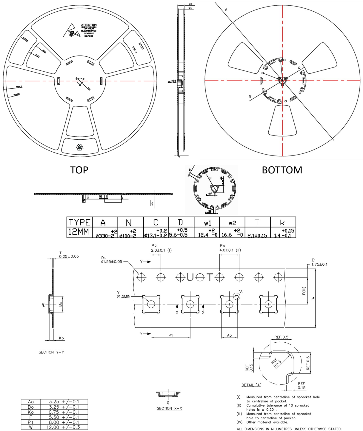
Figure 8: 8TR8217 Tape and Reel Dimension
