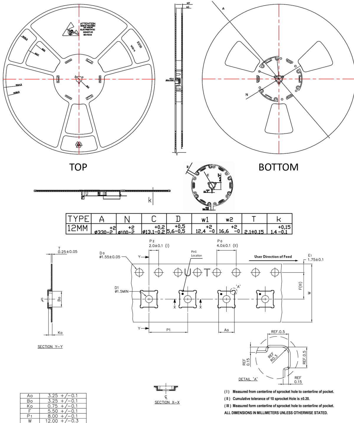
Figure 9. 8TR8217 Tape and Reel Dimension
