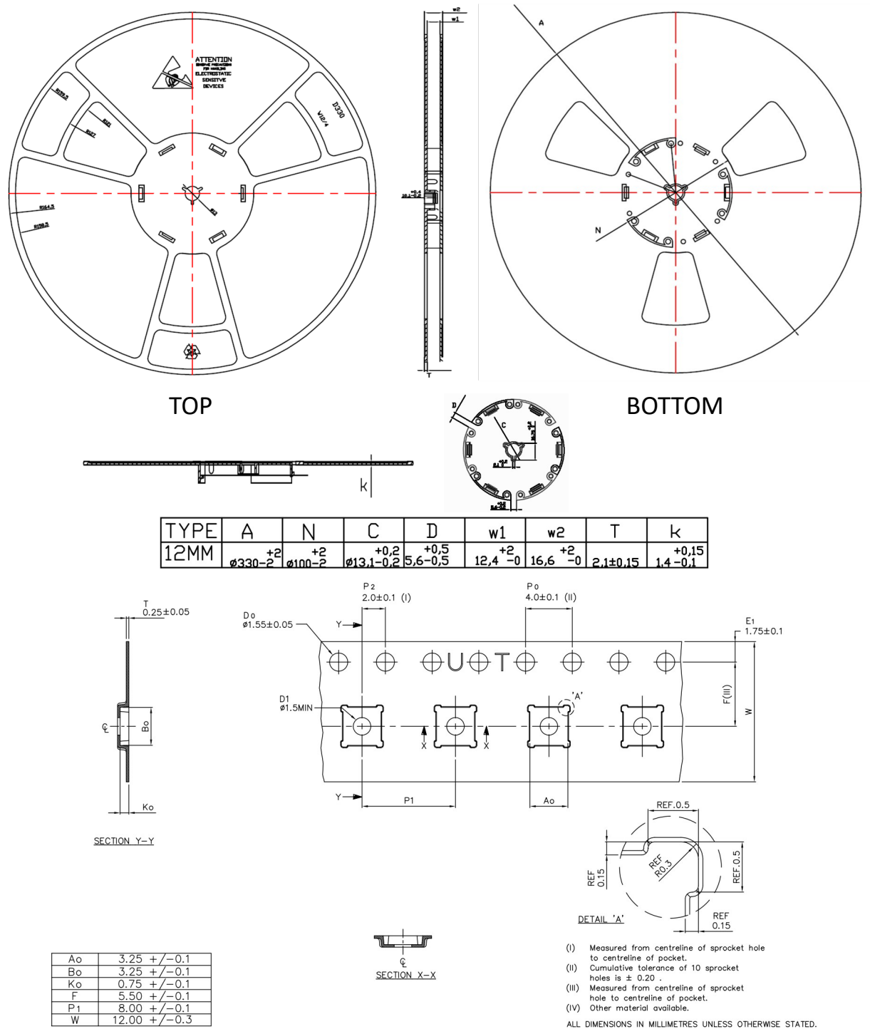
Figure 8: 8TR8219 Tape and Reel Dimension
