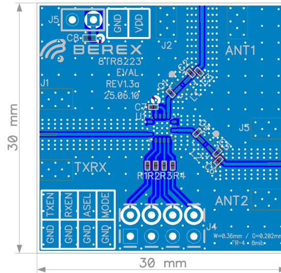
Figure 5. 8TR8223 Evaluation Board PCB Layout
