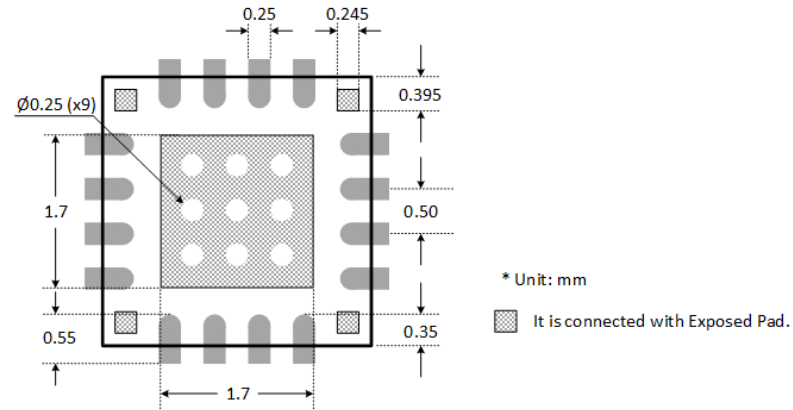
Figure 7. 8TR8223 PCB Layout Footprint
