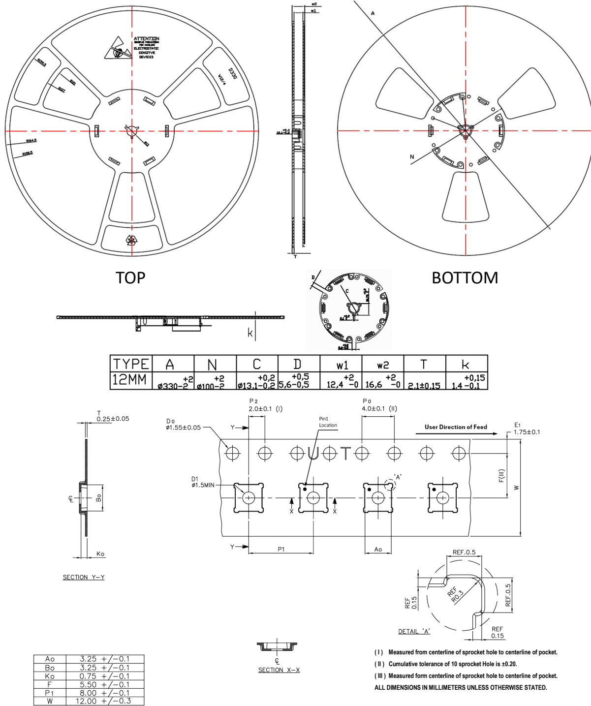
Figure 10. 8TR8223 Tape and Reel Dimension
