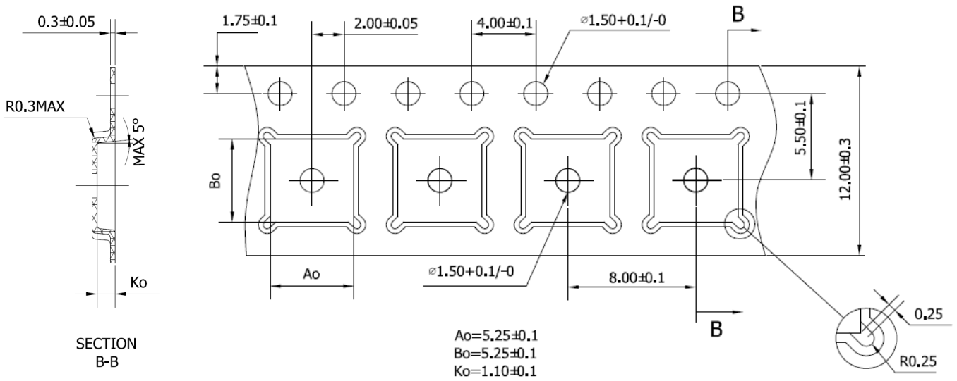
Figure 65. Tape & Reel
