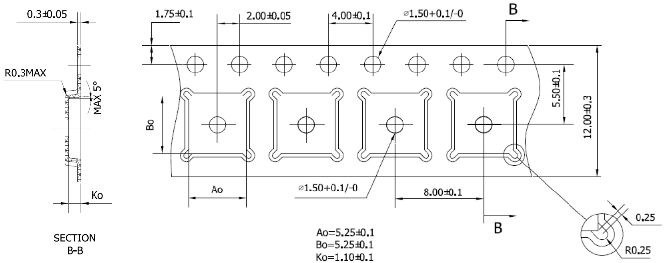
Figure 50. Tape & Reel
