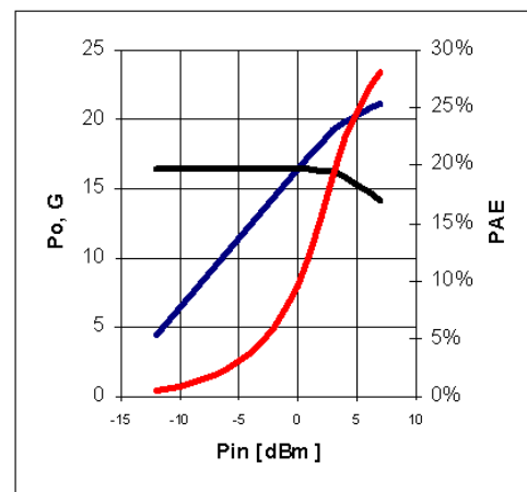
1900 MHz, 5V/85mA
