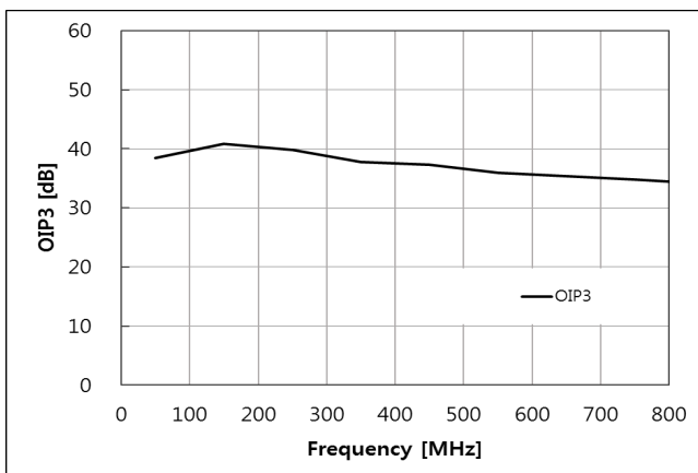
OIP3 vs. Frequency 7dBm / Tone, 1MHz Spacing
