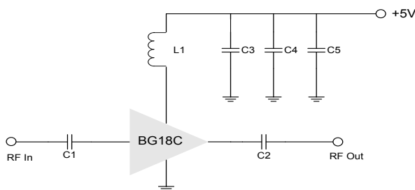
Figure 1 Applications Circuit
