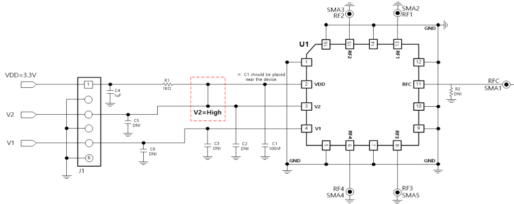
Figure 25 Application Circuit
