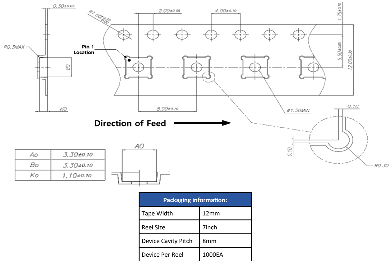
Figure 30. Tape & Reel
