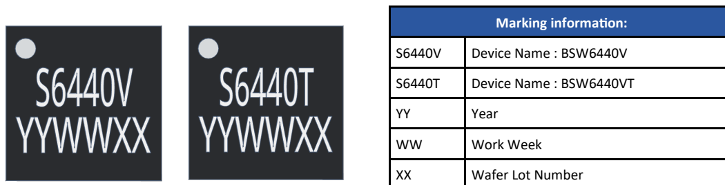
Figure 31. Package Marking
