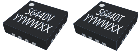
3mm x 3mm x 0.75mm, 16-Lead TQFN Package
