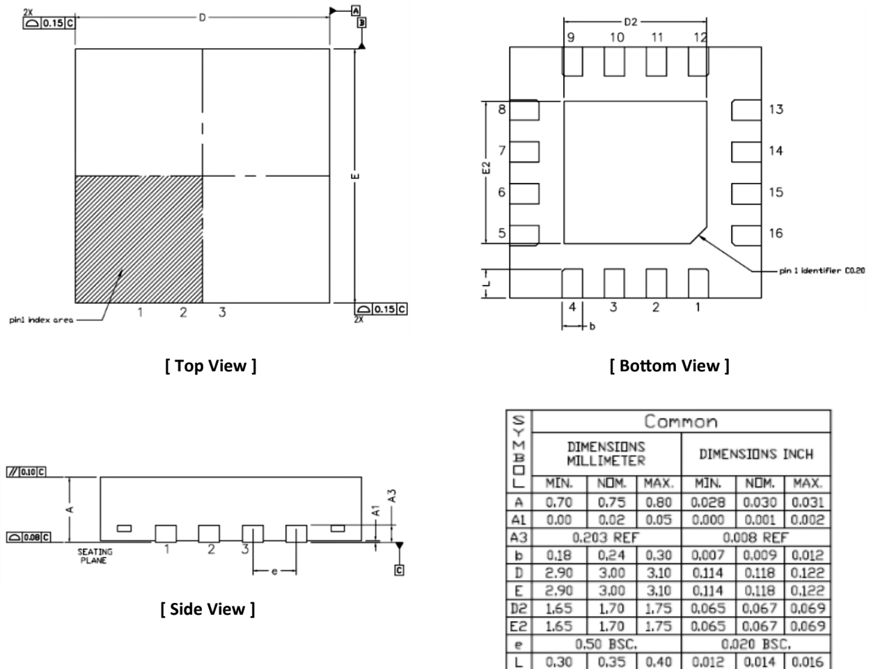
Figure 28. Package Outline Drawing
