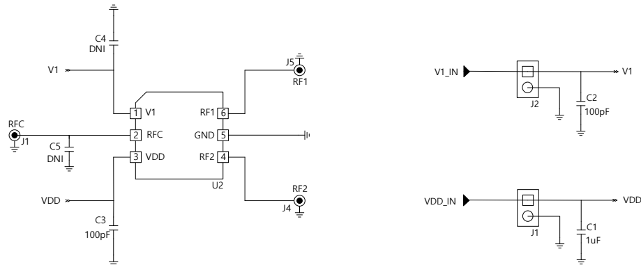
Figure 13. Evaluation Board Schematics
