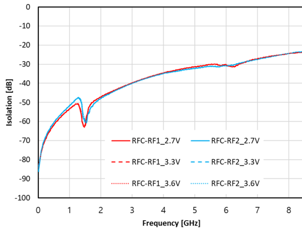
Figure 8. Isolation vs. Vdd (RFC - RFx)
