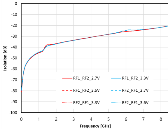
Figure 10. Isolation vs. Vdd (RFx - RFx)
